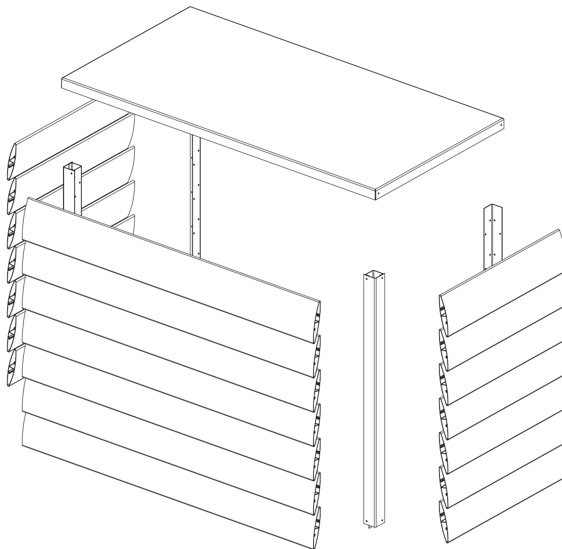
Exploded view, Standard 940.
