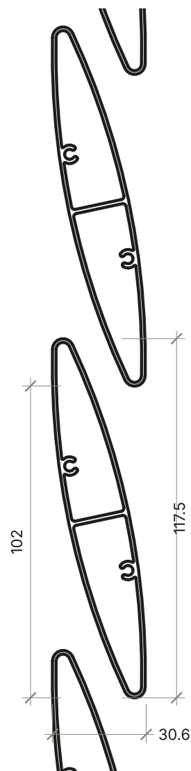
Section through the front louvres, Standard 940. Dimensions in mm.
