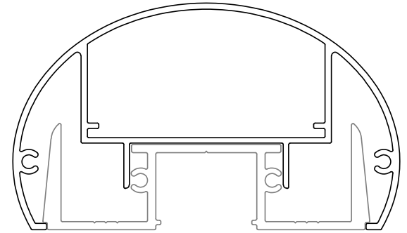
DIE No.TR-R4080 | ELEGRA ROUNDED HANDRAIL
