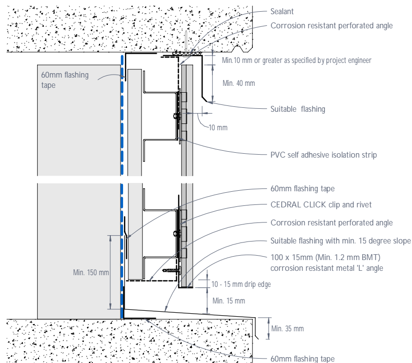
Figure 23: CEDRAL CLICK junction with exposed concrete slab or beam - Cladding recessed
