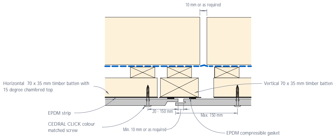
Figure 4: CEDRAL CLICK vertical control joint - Detail 1
