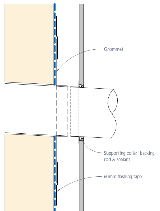
Figure 31: Pipe penetration - Section
