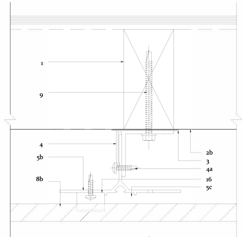
2 Intermediate Support 01-01 205 1:2 @ A3
