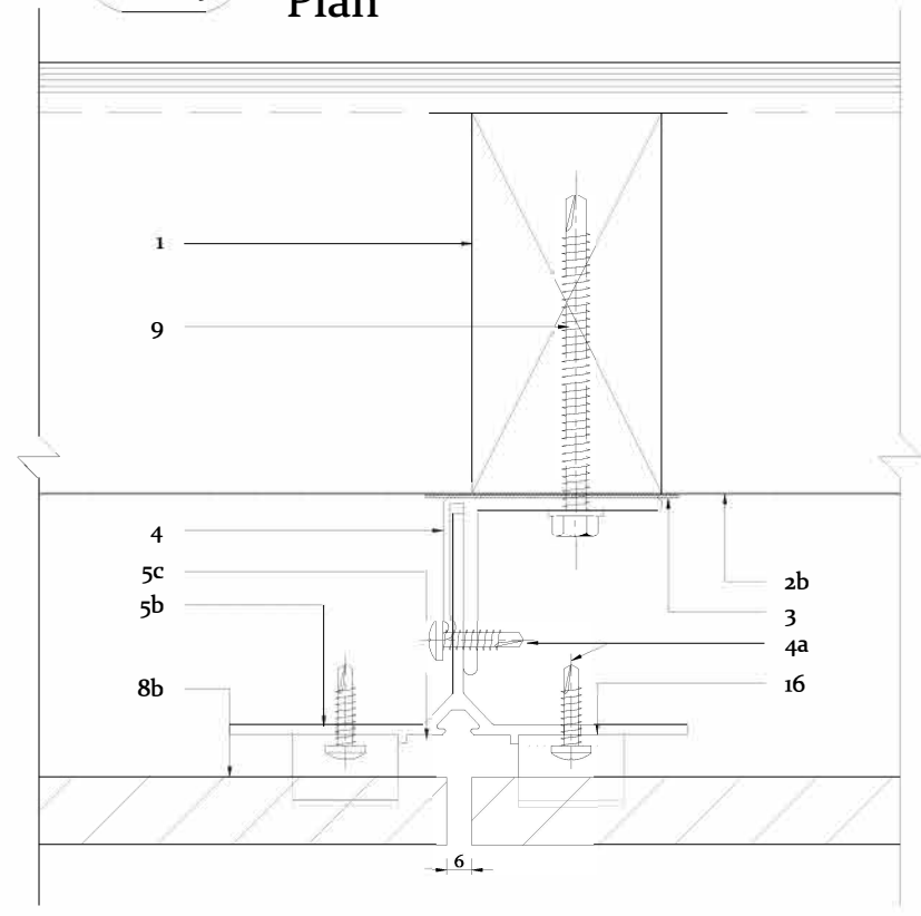
1 Negative Detail 01-01 205 1:2 @ A3
