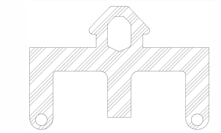
SCALE - 2:1 @ A3 EPDM-BR-E6J Length = 2990 ±mm Dimension tolerance basis: NF ISO 3302 (E2) Material : EPDM DS70 MP Std 2710
