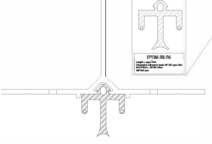
support profile + Joints EPDM-BR-E6
