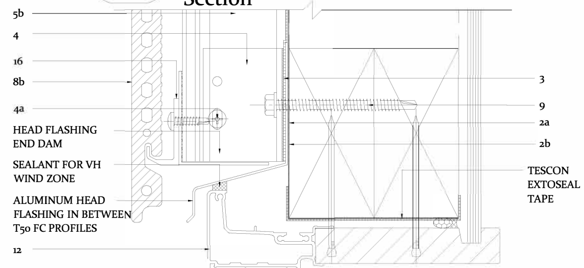
3 Window Head Detail 01-01 205 1:2 @ A3
