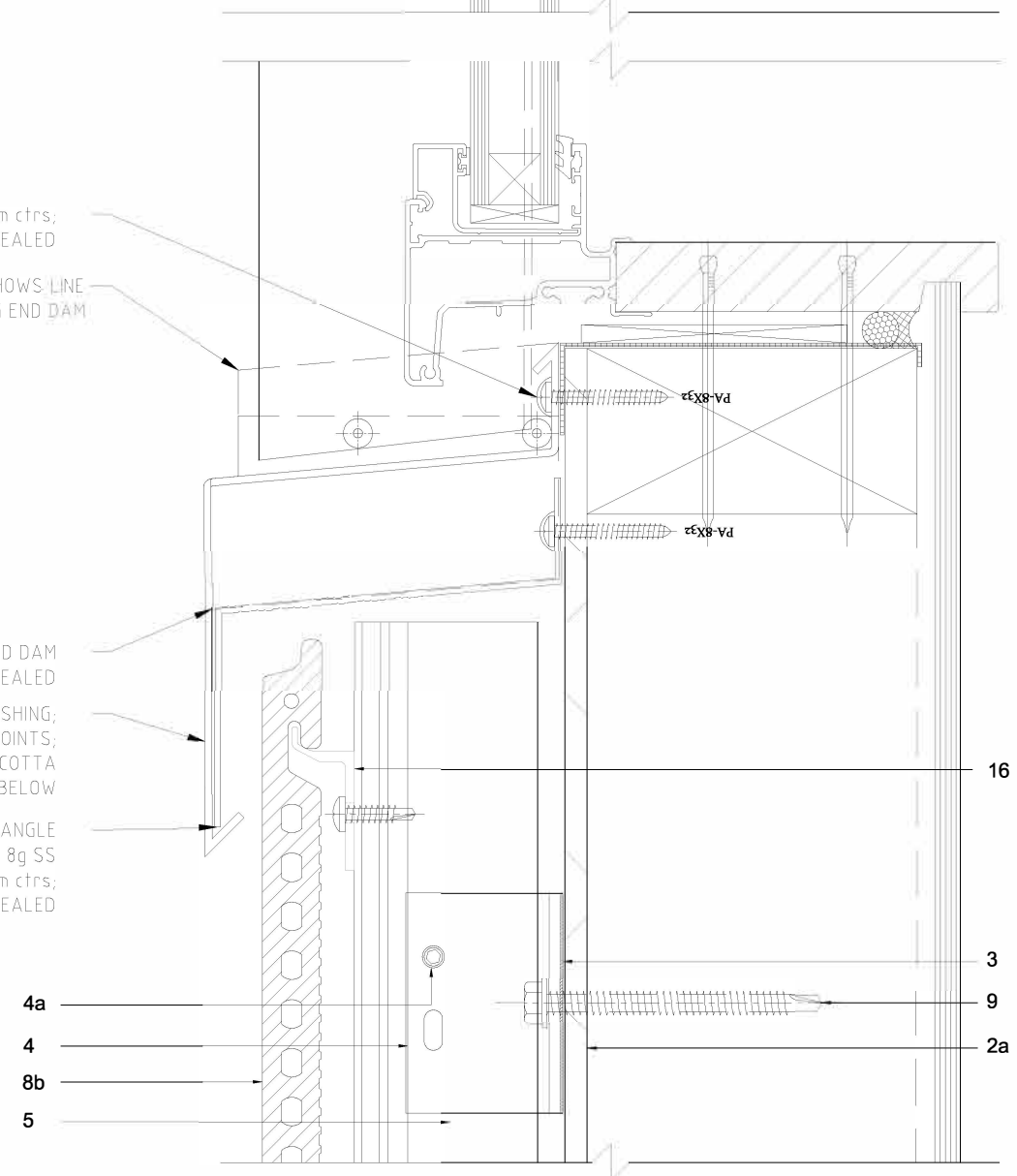
4 Window Sill Detail 01-01 205 1:2 @ A3
